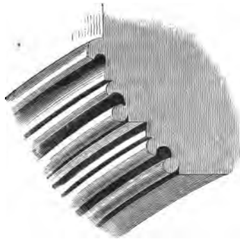
72. Nave of Milton Church, Oxon. Arch-mouldings.
